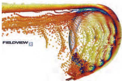
CFD Particle study showing harmonic shedding of airflow. This phenomenon is perceived by the rider as 'buffeting' was critical to solving the stability and handling aero wheels during the Firecrest development.
