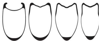
303 Firecrest Carbon Clincher
