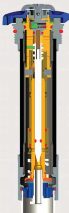
Rebound Assembly
