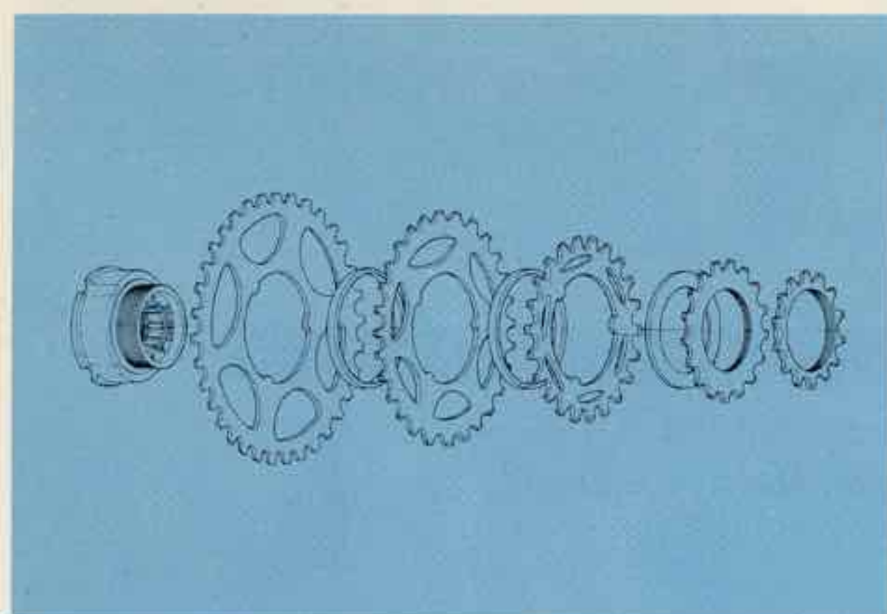
Exploded view
