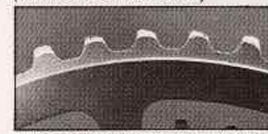
Front Chainwheel after shifting 10,000 times. (With use of Conventional Chain)
