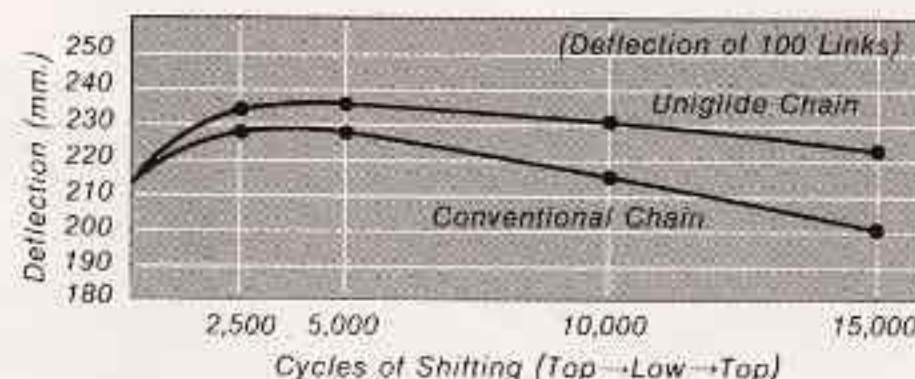
Graph. 1: Deflection of Chain After Repeated Gear Shifts
