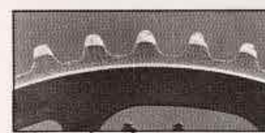
Front Chainwheel after shifting 10,000 times. (With use of UG Chain)
