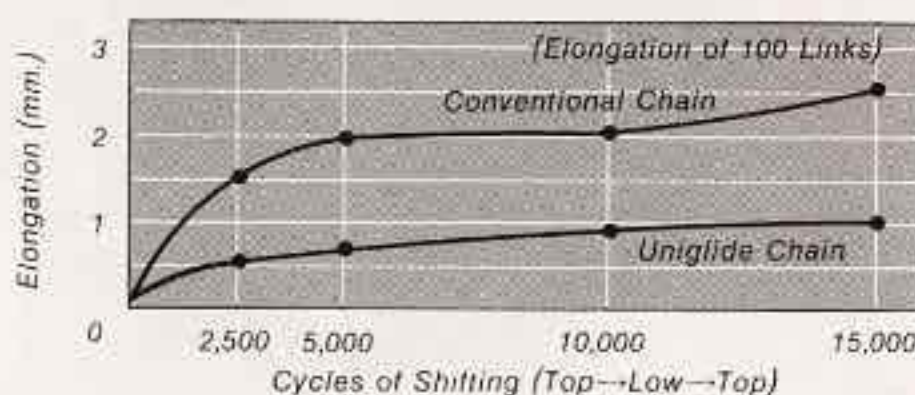
Graph. 2: Elongation of Chain After Repeated Gear Shifts
