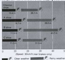
Comparison Test of Different Shoes' Stopping Distances
