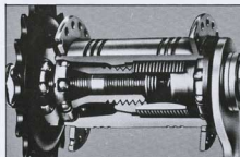
Sectional View of Coaster Brake
