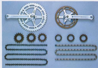
DURA-ACE 10 — DURA-ACE Comparison Photo
