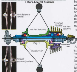
• Conventional Dura-Ace Hub & Freehub
