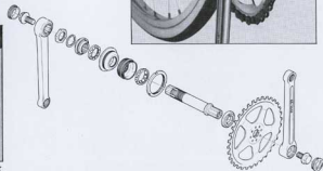
OCTA Joint Crank
