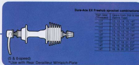
Freehub
