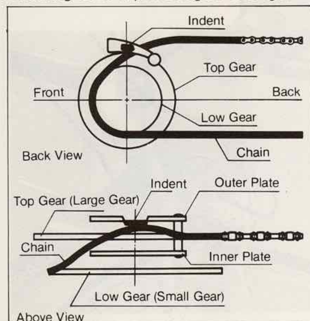
Chain Protector Release Indentation's movement
