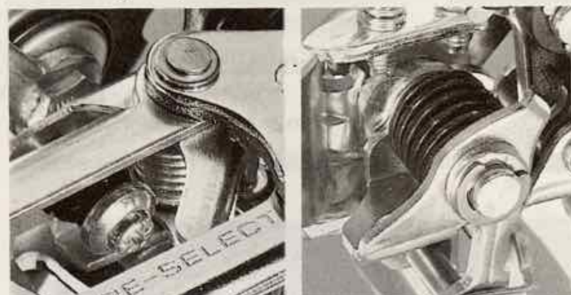
Pre-Select Mechanism on Positron-II Rear Derailleur
