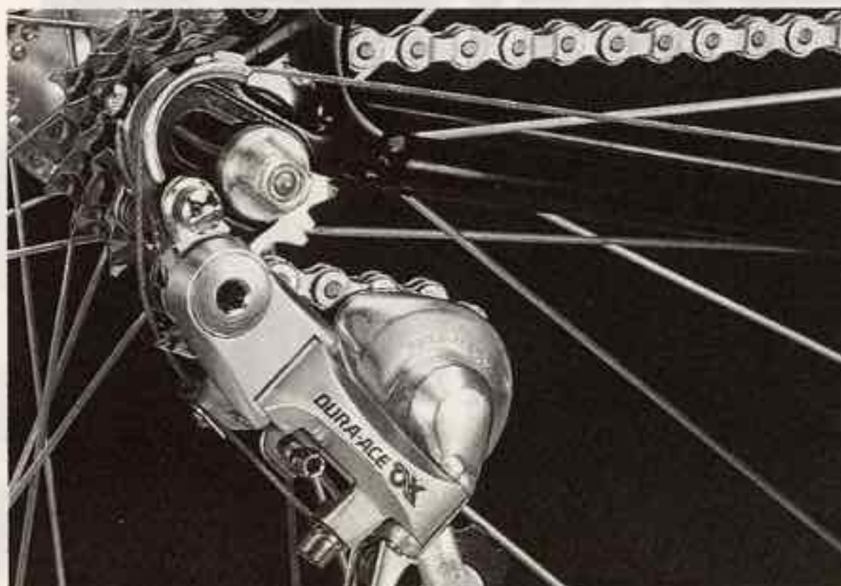
Direct Cable Mechanism
