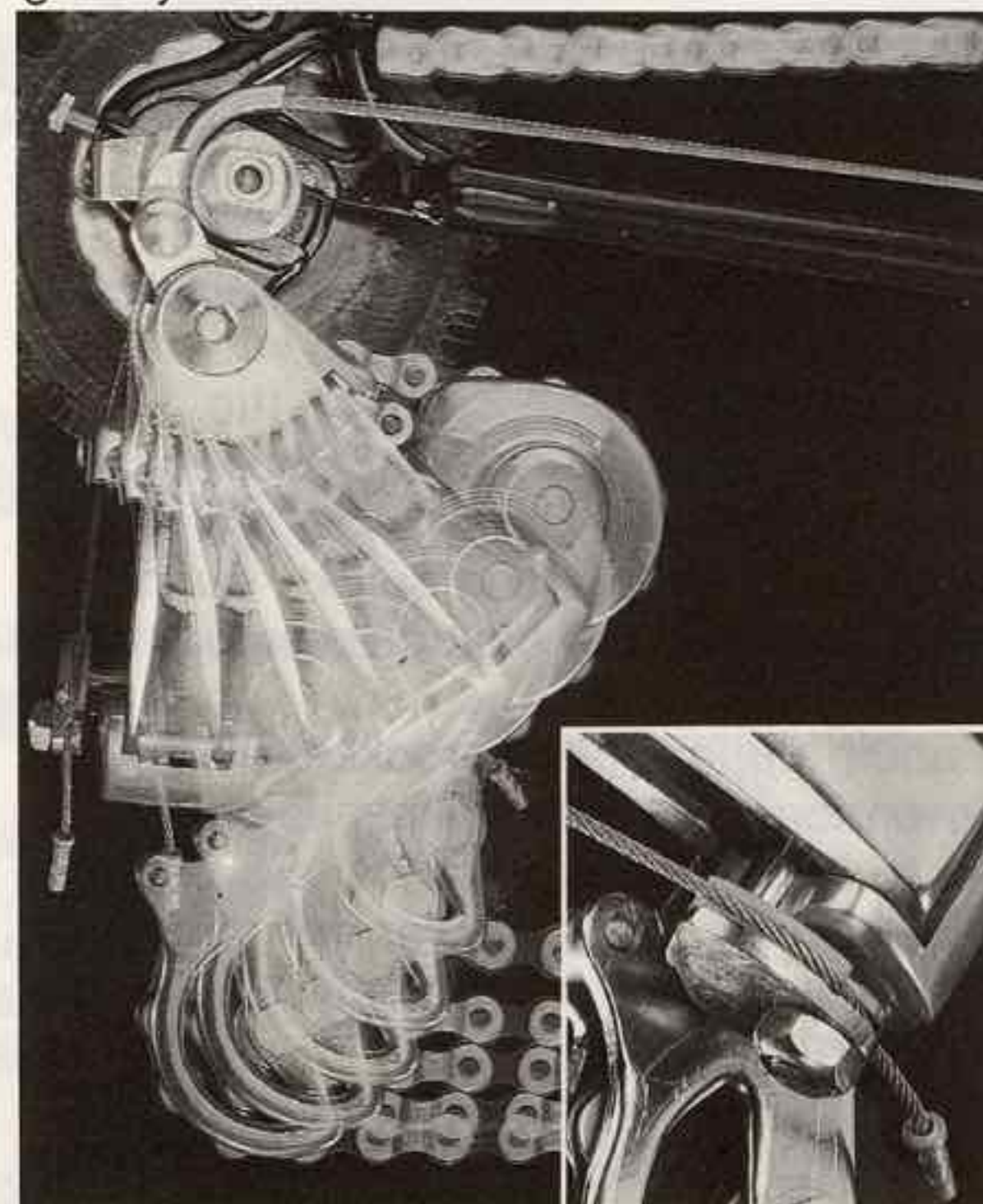
Pre-Select Mechanism and Rear Derailleur's Movement
