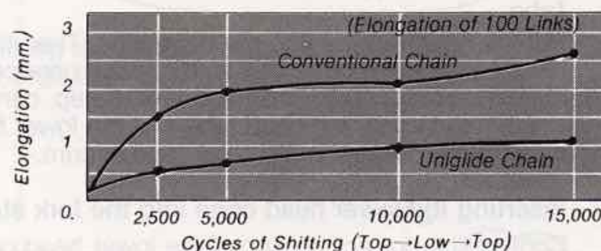
Graph 2: Elongation of Chain After Repeated Gear Shifts
