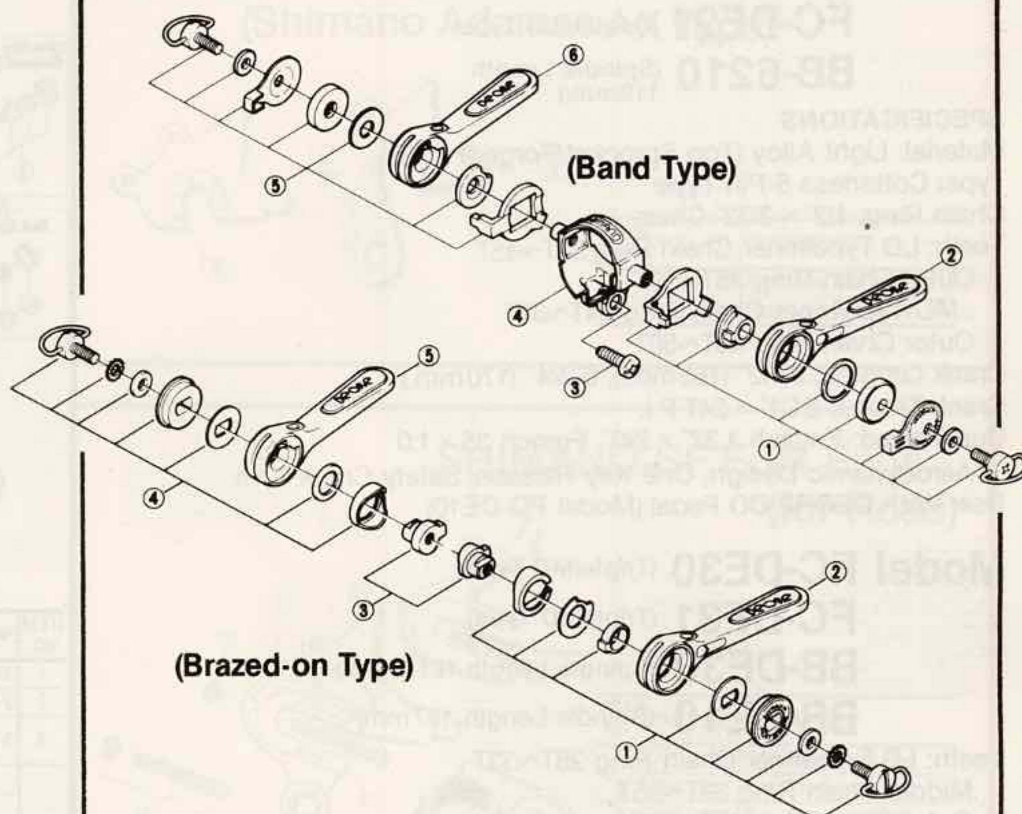
(Band Type)
