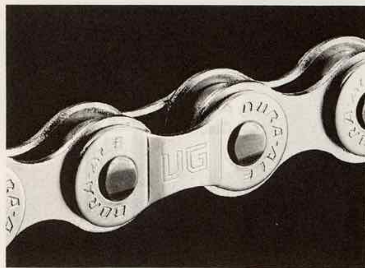
The UG Chain. Outerplates are widened to the level of chainpin heads.
