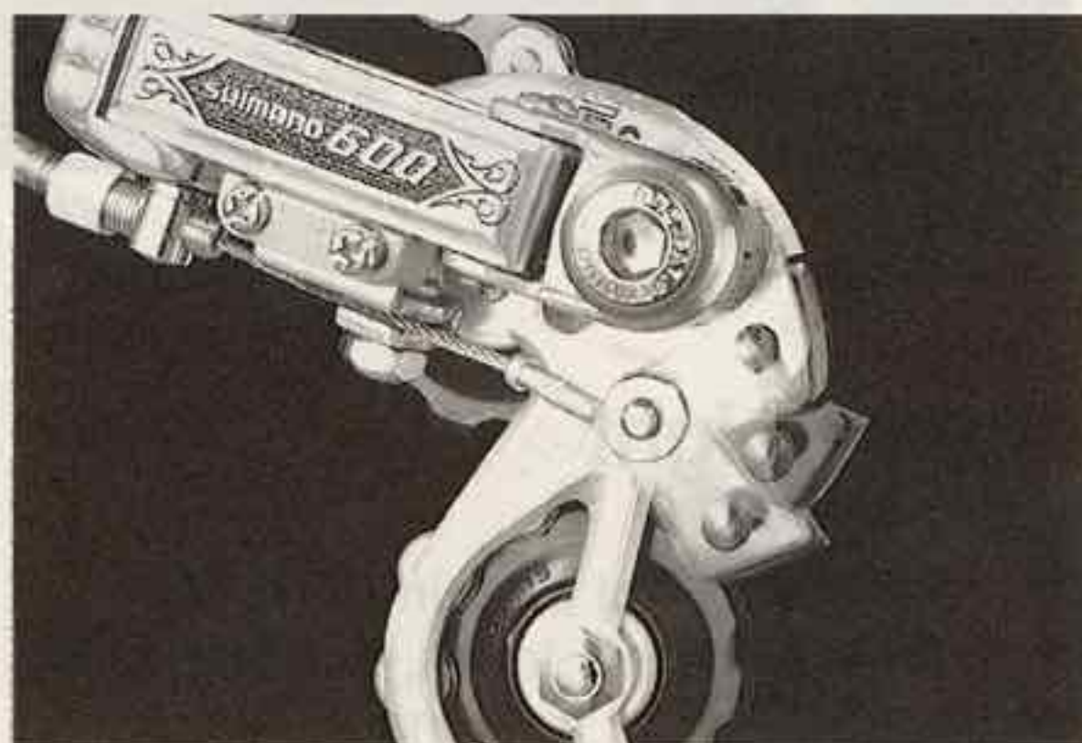
Hatch-Plate Mechanism
