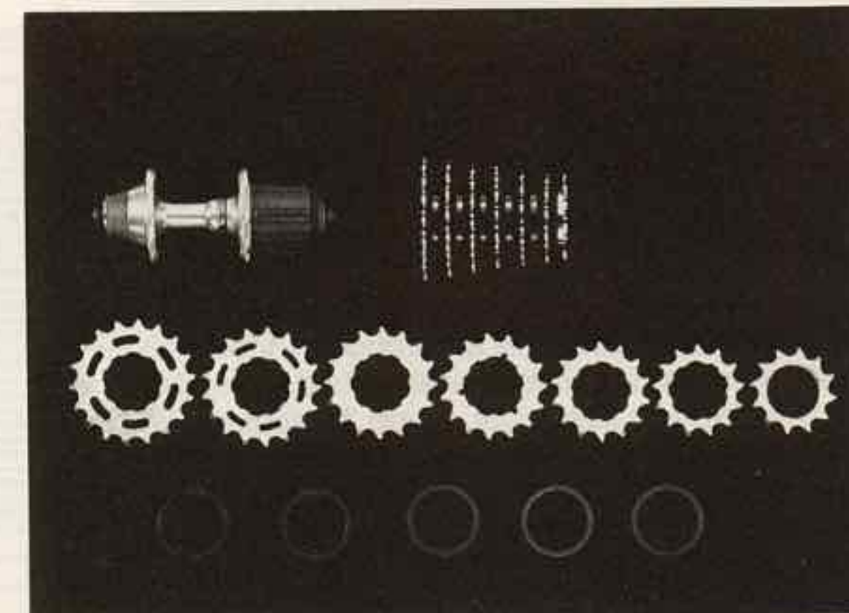
Top gear is threaded style with second spline type.
