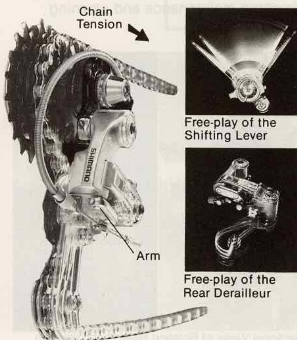
Chain Tension
