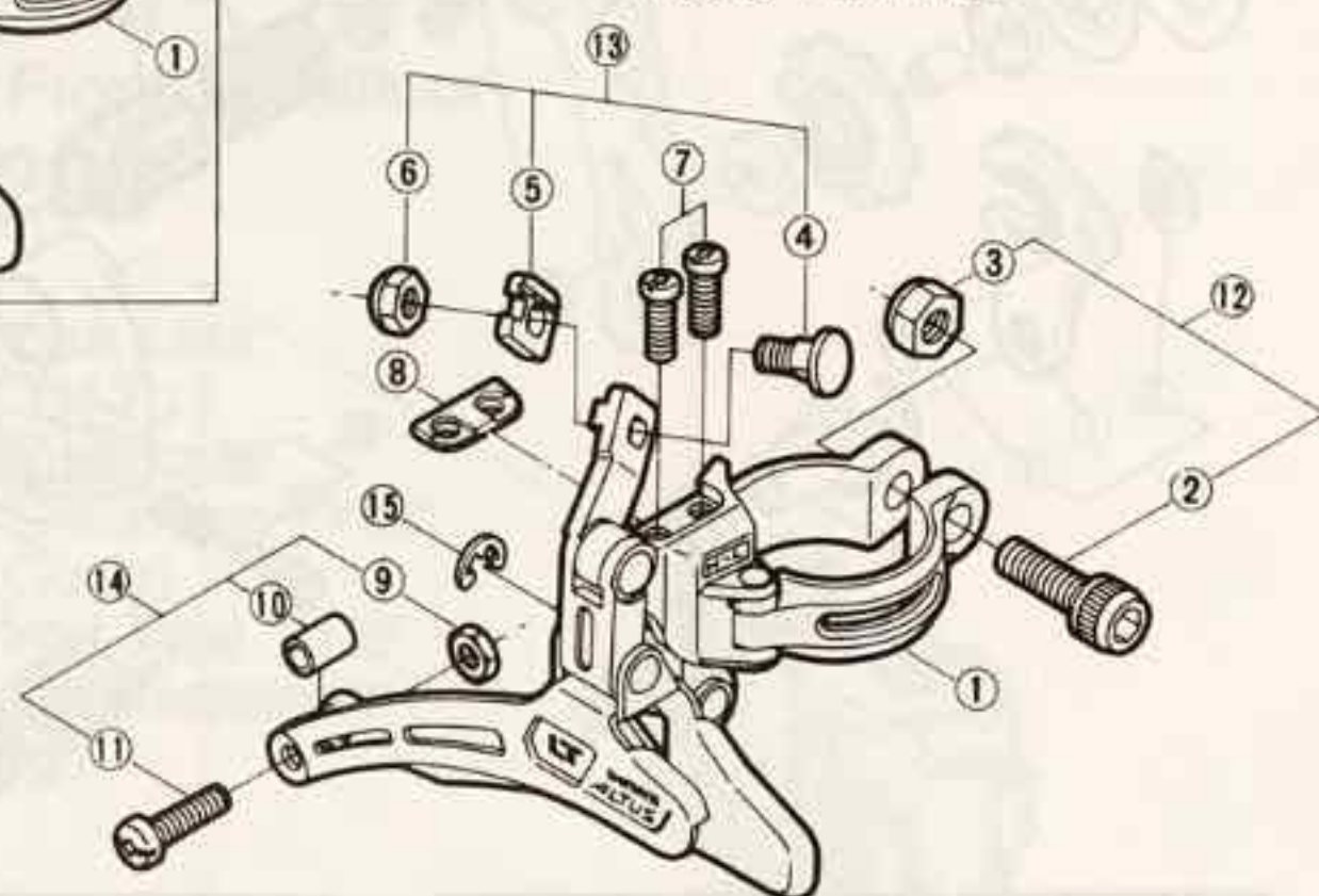
ALTUS-LT Model FD-AT12
