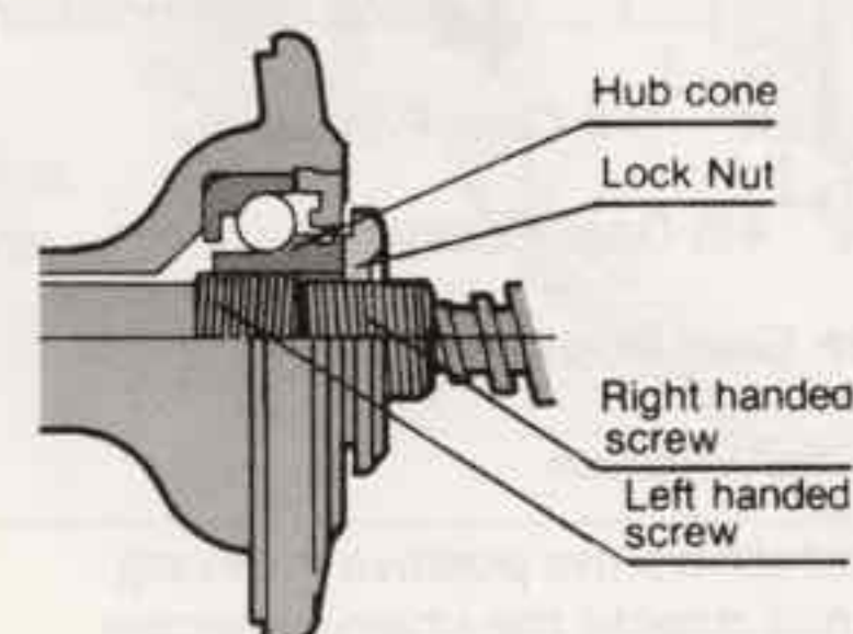
Special Front Hub Axle Structure
