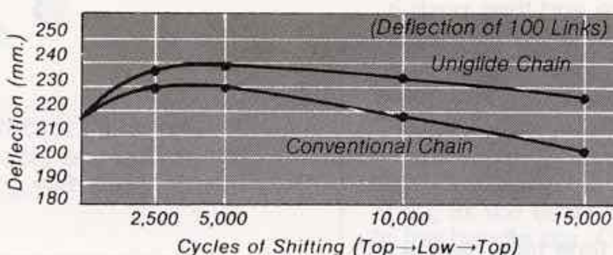
Graph 1: Deflection of Chain After Repeated Gear Shifts
