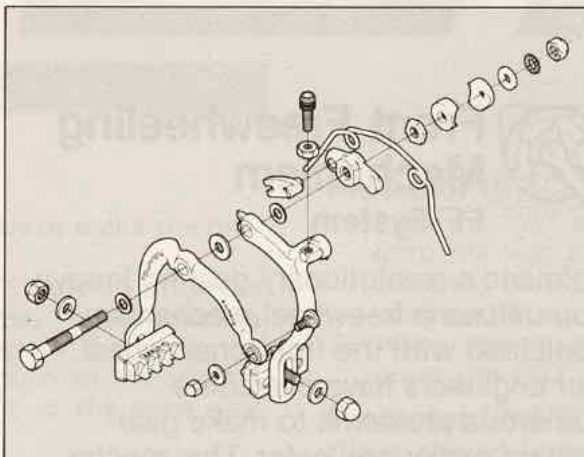
The ideally shaped Chevron Shoe—the result of Shimano's numerous brake tests.
