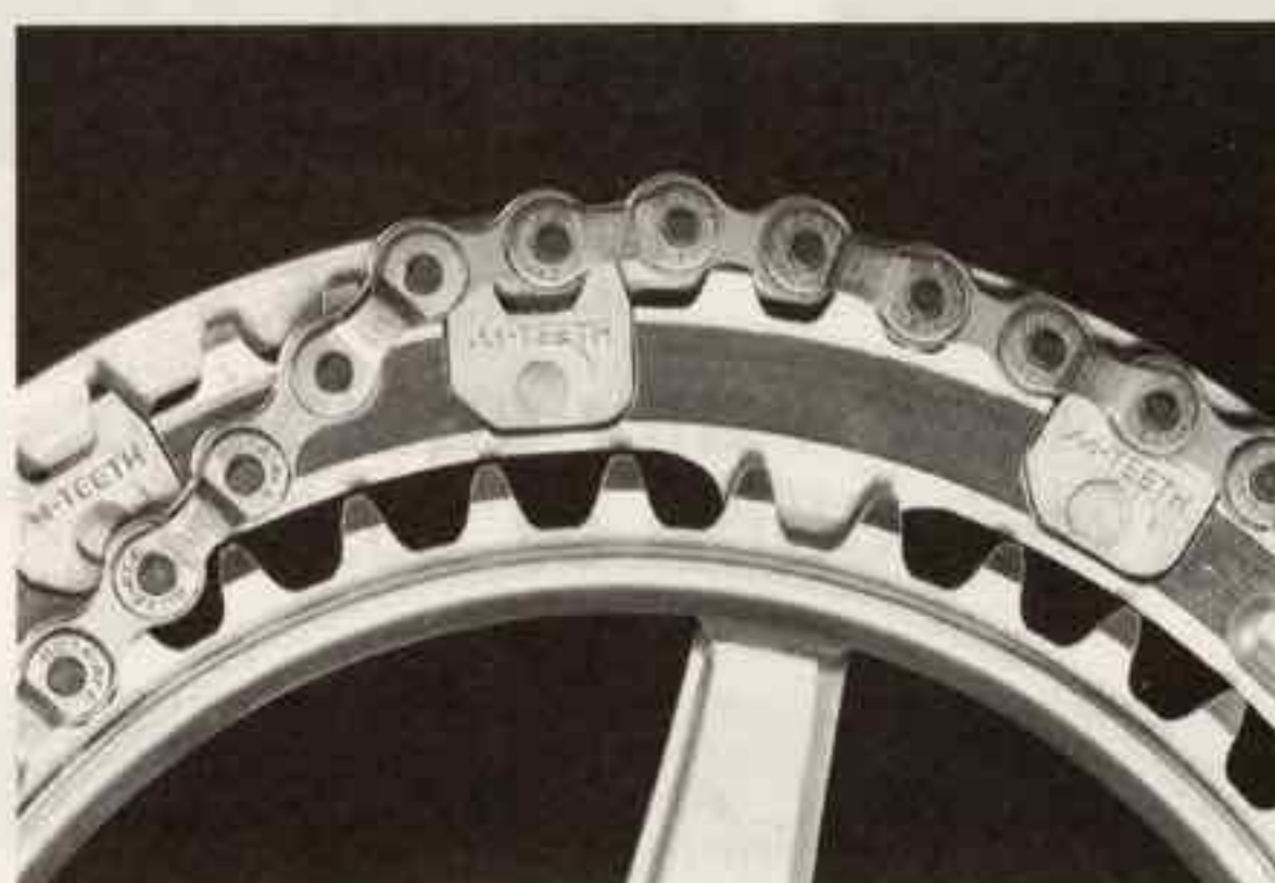
The Chain on Front Chainwheel with aligned large and small gears.
