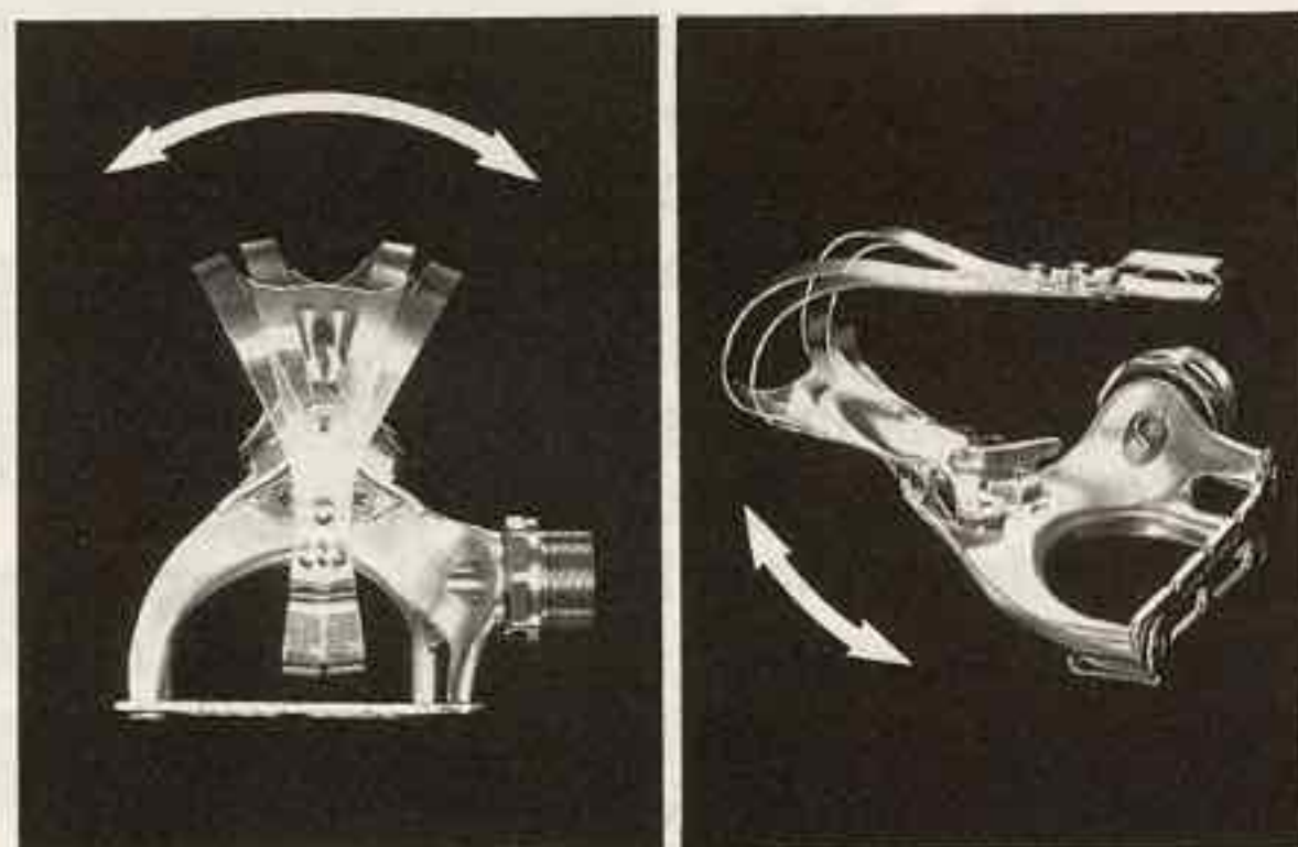
DD Pedal The toe-clip adjusts back and forth by 10mm (0.39"), and also laterally to obtain the most comfortable setting.
