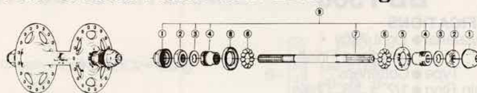
Front Hub
