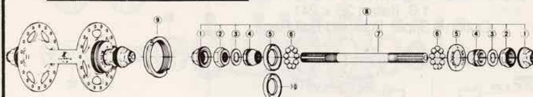
Rear Hub (OVER LOCK NUT DIMENSION 110 mm)
