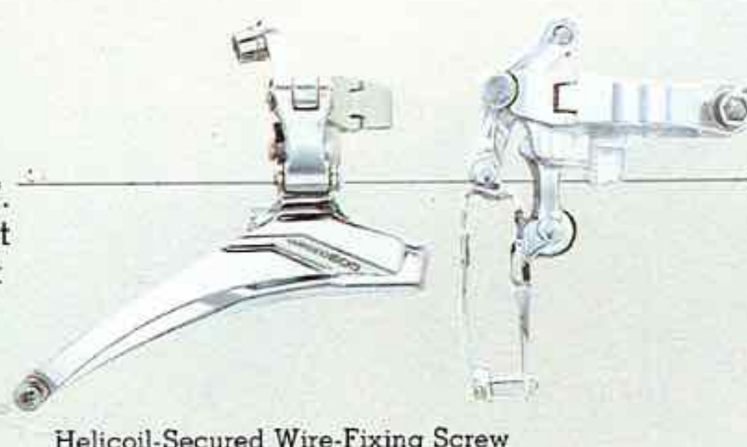
Helicoil-Secured Wire-Fixing Screw
