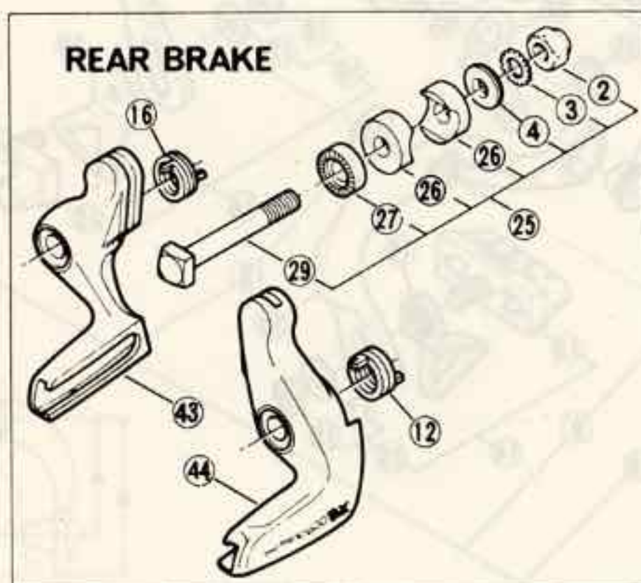
BR-6310
