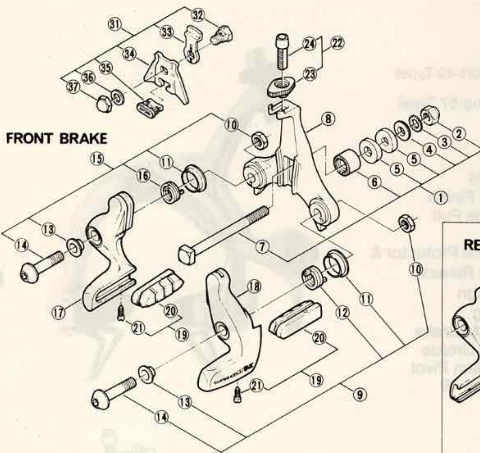
BR-6300
