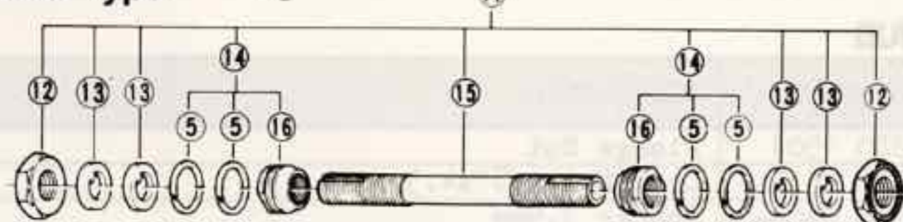
Quick Release Type
