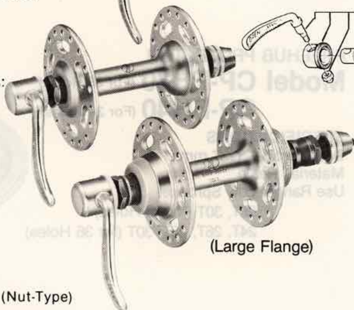
(Small Flange)
