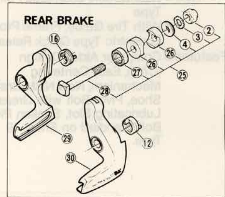
BR-6300
