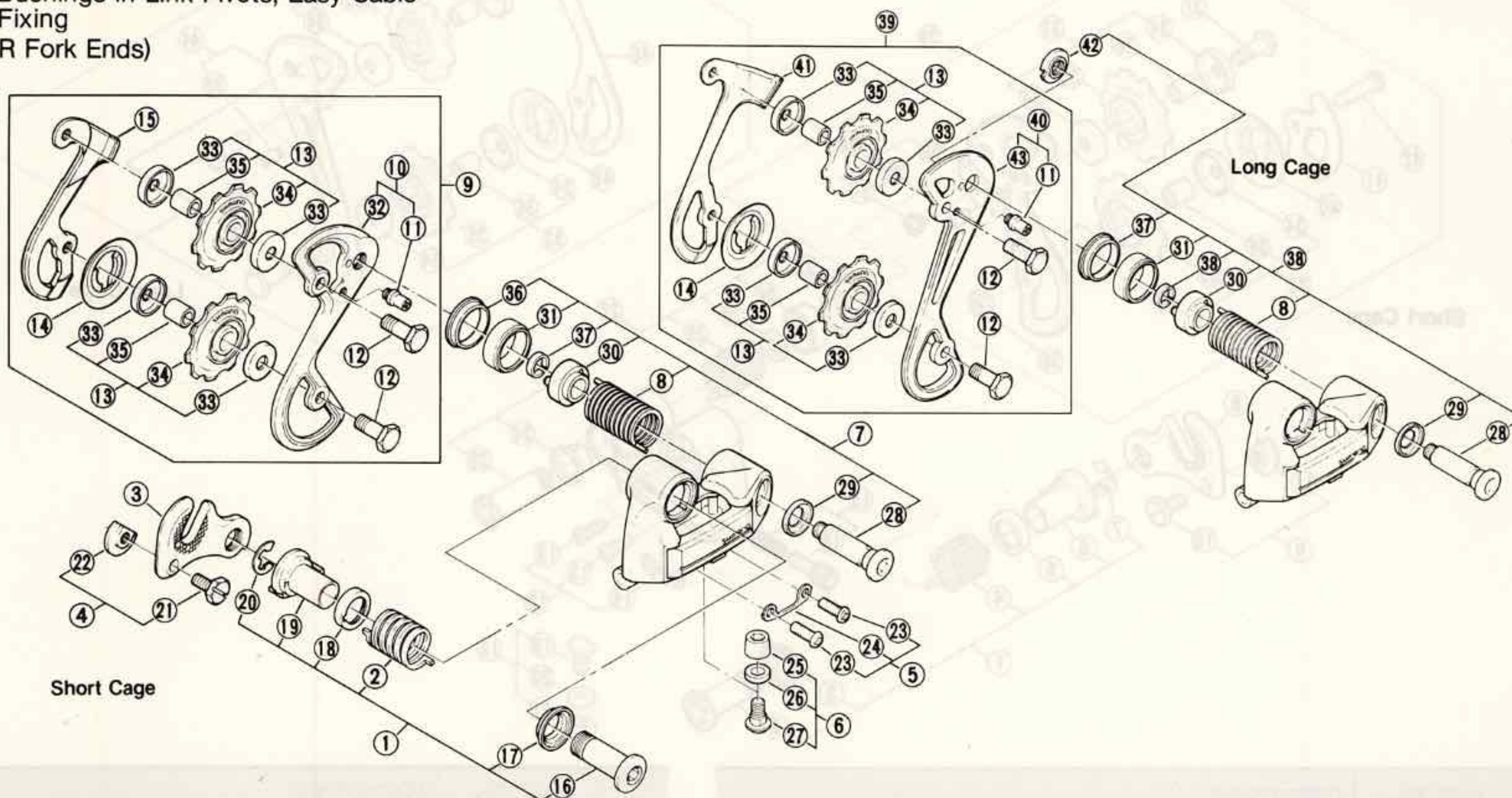
(Short Cage)
