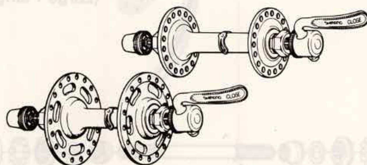
■ Front Hub Over Lock Nut Dimension : 100mm(3-15/16")
