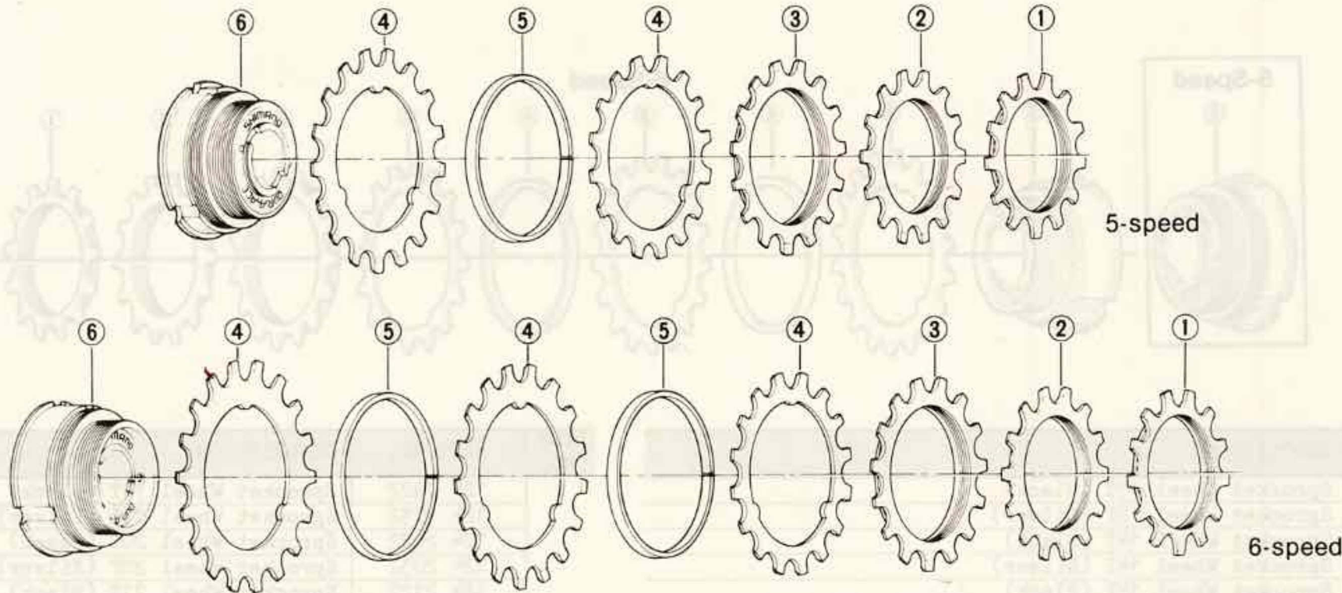
6-speed
