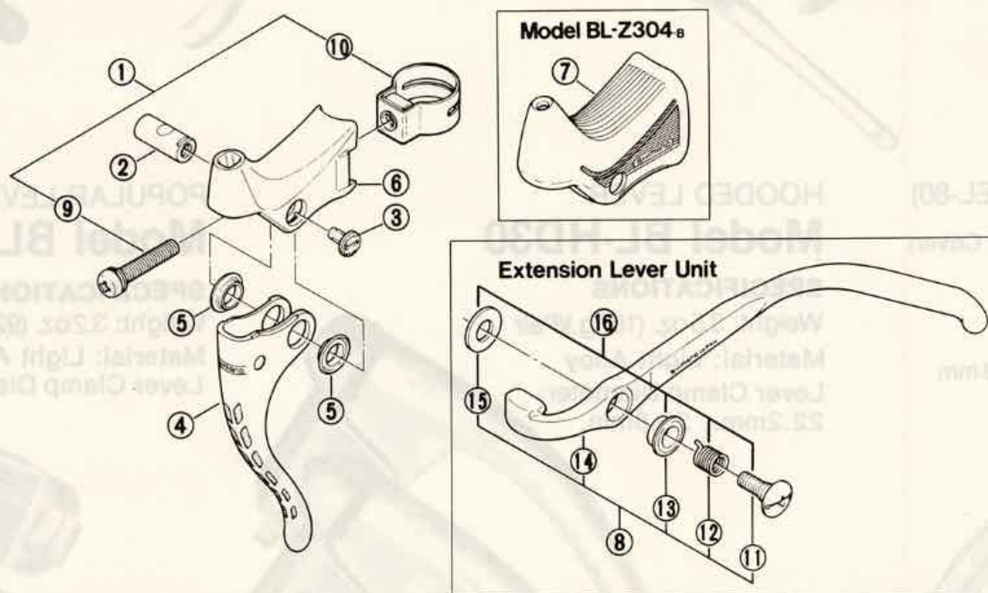
Extension Lever
