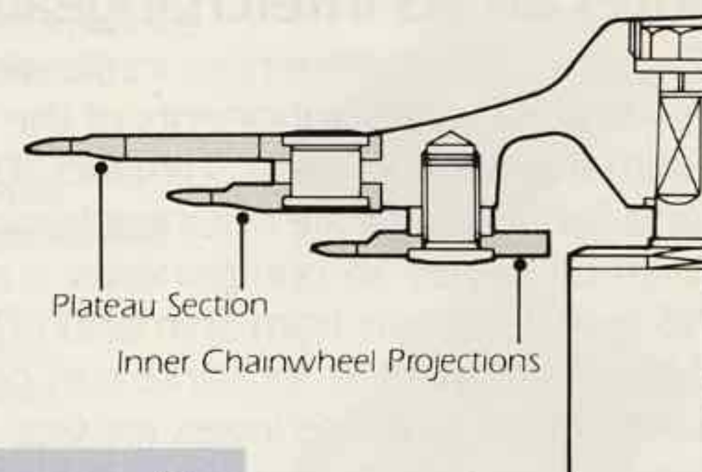
3 Tooth Profiles
