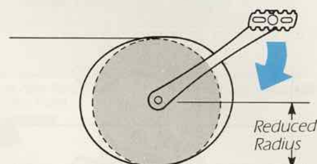
Chainwheel radius is reduced during the downstroke.
