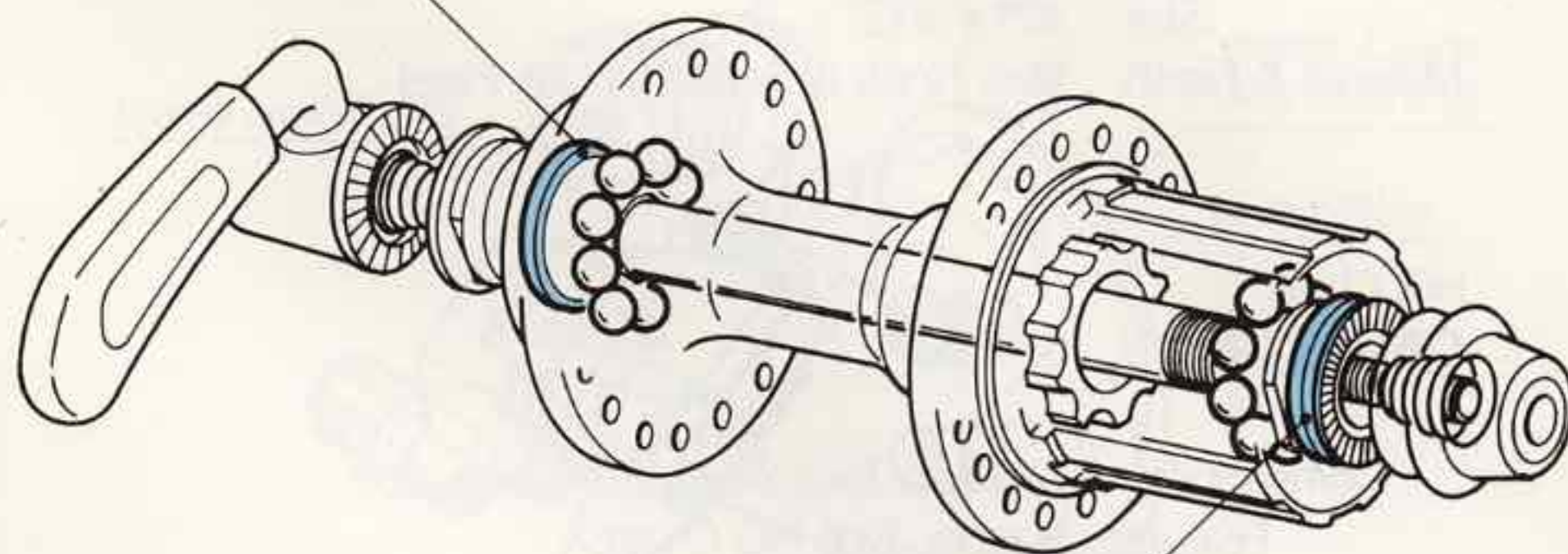
Lip Type Sealed Mechanism
