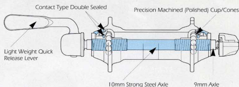
Front Hub HB-M564
