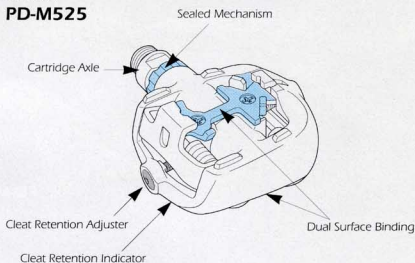
SPD Pedal PD-M525
