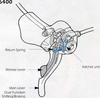
Dual Control Lever SD-6400
