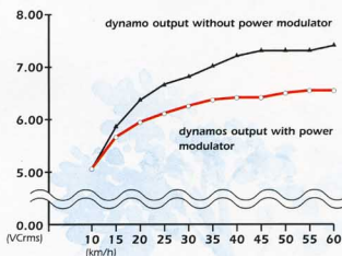
Power modulator (elastomer)
