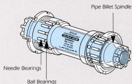
Bottom Bracket (BB-7700)
