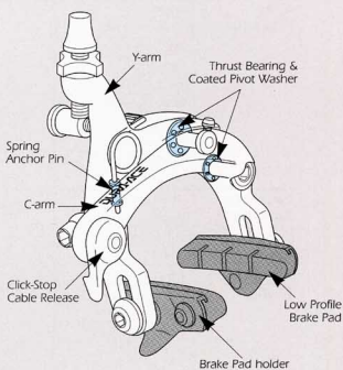
Dual Pivot Brake Caliper (BR-7700)
