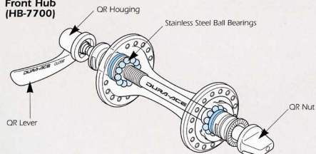
Front Hub (HB-7700)
