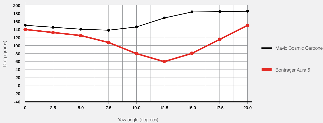
Aerodynamic drag—Bontrager Aura 5 vs. Mavic Cosmic Carbone
