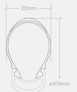
CFD-aided 22c elongated profile
