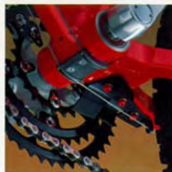
Klein's tradition of innovation includes its patented Chain Control Device™, standard on all 1992 mountain bikes. The device keeps the chain from slipping up between the chain ring and chainstay by sweeping it clean and avoiding chain suck.
