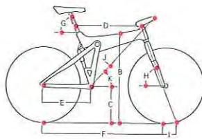
Mantra Series frame Line drawings correspond to chart dimensions.
