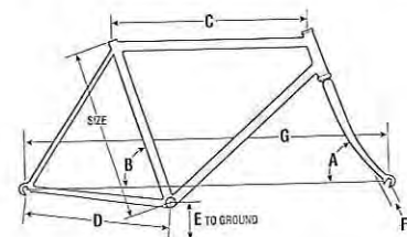
Frame Geometries: MultiTrack and Road Bikes
