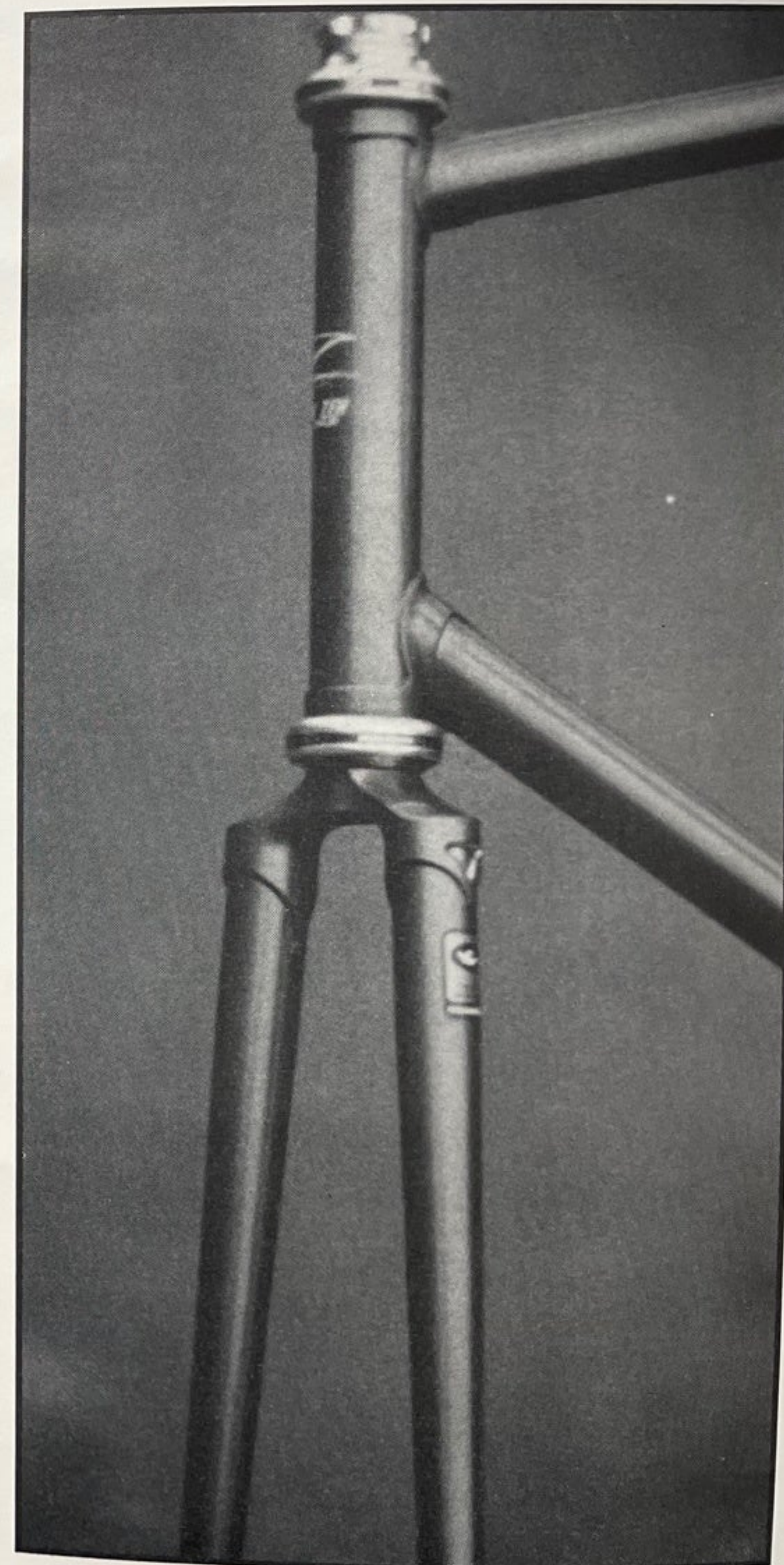
bottom: Fat, 24mm track blades are used in this SLX™ track frame, rather than the less rigid 22mm blades commonly used.
