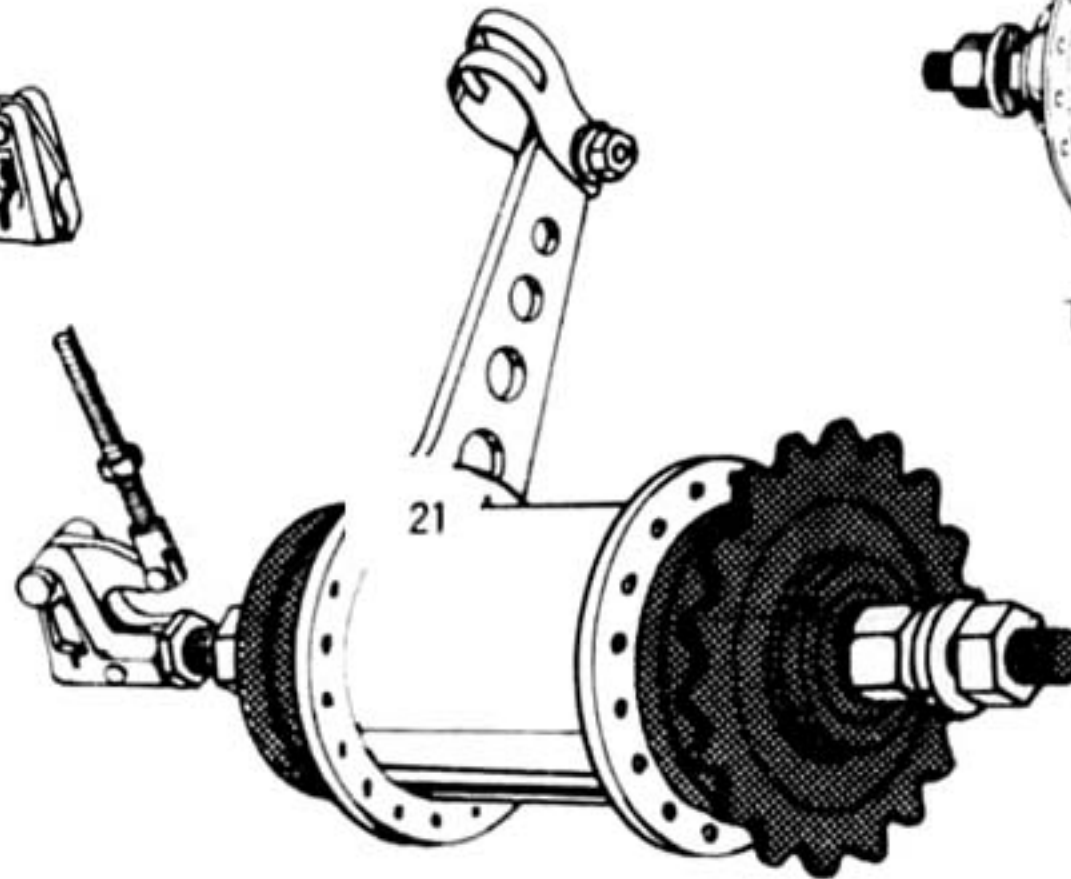
"Shimano" 3-Speed Coaster Hub
