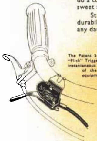
AM Three-speed Hub medium ratio with Handlebar "Flick" Trigger Control. 15.55% increase, 13.46% decrease from normal. Suitable for sports and racing Bicycles.
